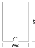
Controcassa Outercasing
